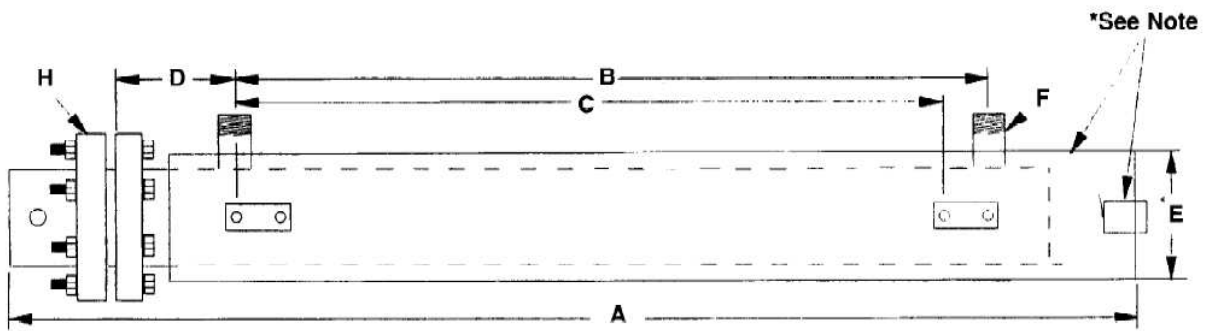
Figure 1: Threaded Connections
