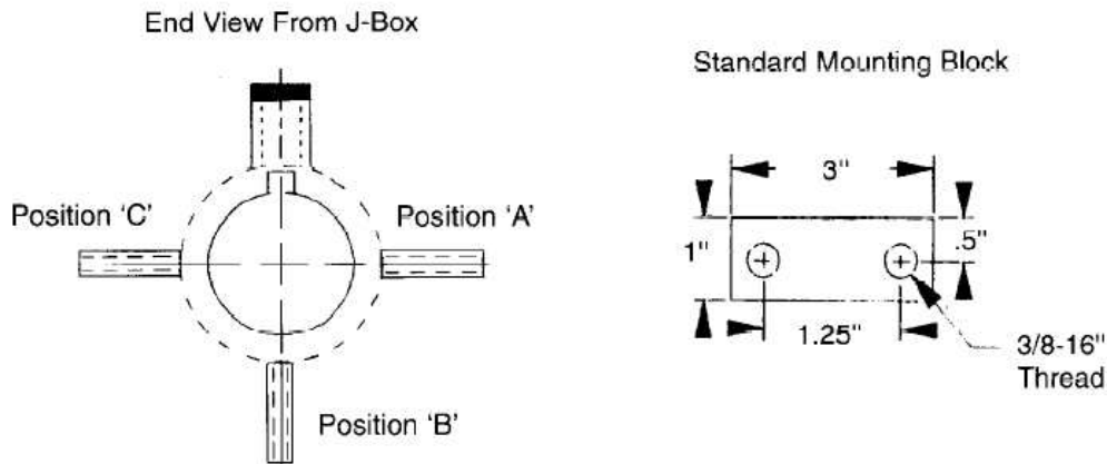
Figure 1: Threaded Connections
